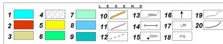
Lithological-structural cross section along AA1 line
