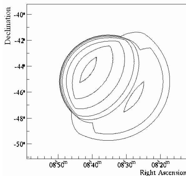
Fig. 2. Simulated brightness temperature map of the Vela SNR at 408 MHz.
