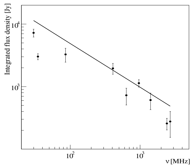
Fig. 1. Integrated flux density spectrum.
